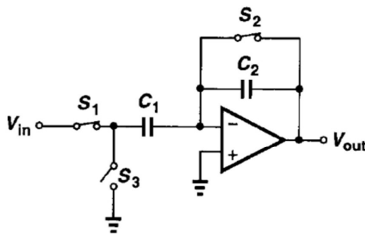
Figure 12.4 Switched-capacitor amplifier.
