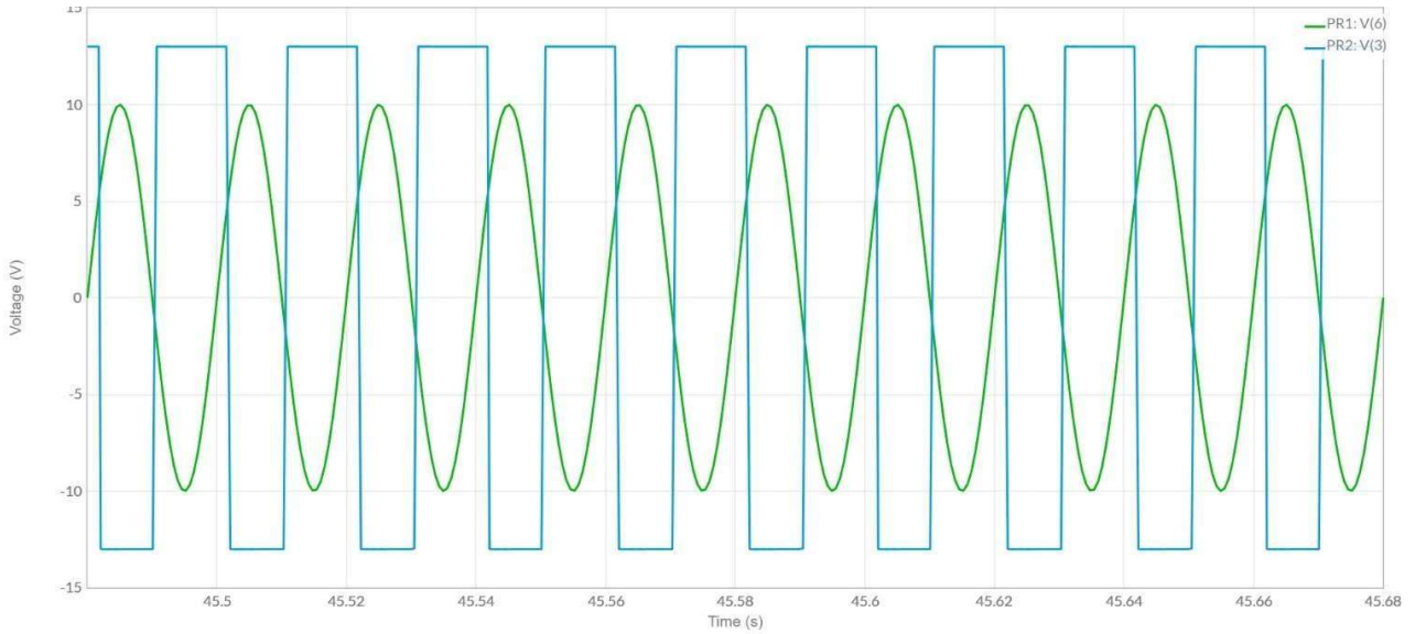
Fig. 3: Output Waveform of Bistable Multivibrator Circuit in Multisim
