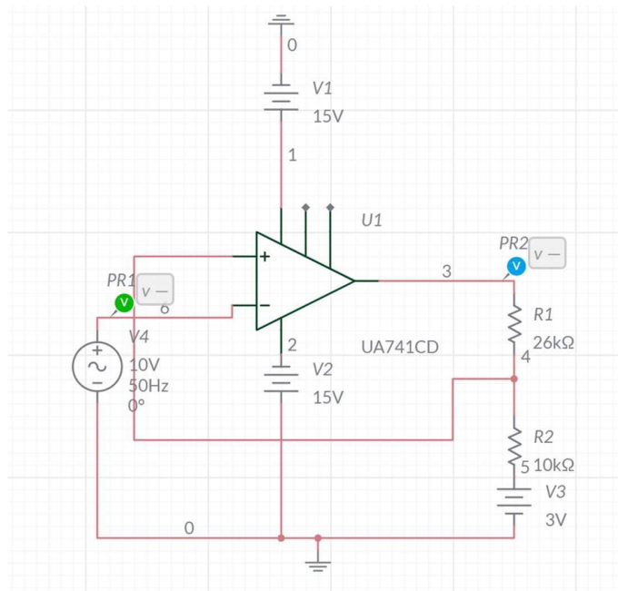
Fig. 2: Bistable multivibrator Circuit in Mutisim
