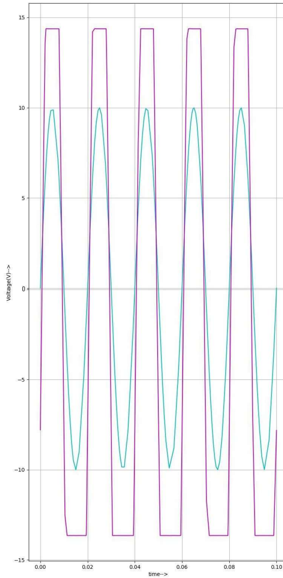
Fig. 5: Output Waveform Bistable multivibrator Circuit in Esim
